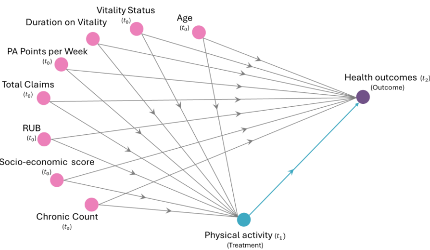
Figure 4: Directed acyclic graph
